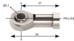
# 62.527 Ball Swivel End M5x27
