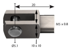
#62.520 Fork with pin M5x20
