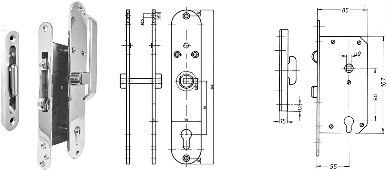
SET: 13.9699Z Heavy duty sliding door lock set for 1 1/2 inch thick doors. Chrome plated brass.
