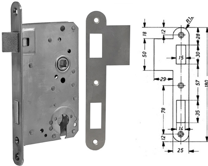
#14.4610.508 Heavy Duty Stainless Steel 65 mm backset Weather Door Entry Lock with solid latch bolt
