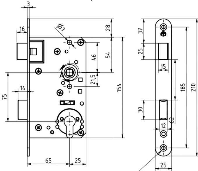
#14.4610.508 65 mm backset. Satin or Polished Stainless Steel DIN 74-Am5
