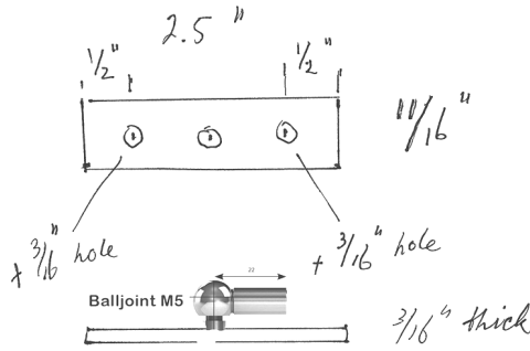
Polished Stainless Steel Bracket # 64.615 for 6-15- stainless steel gas springs
