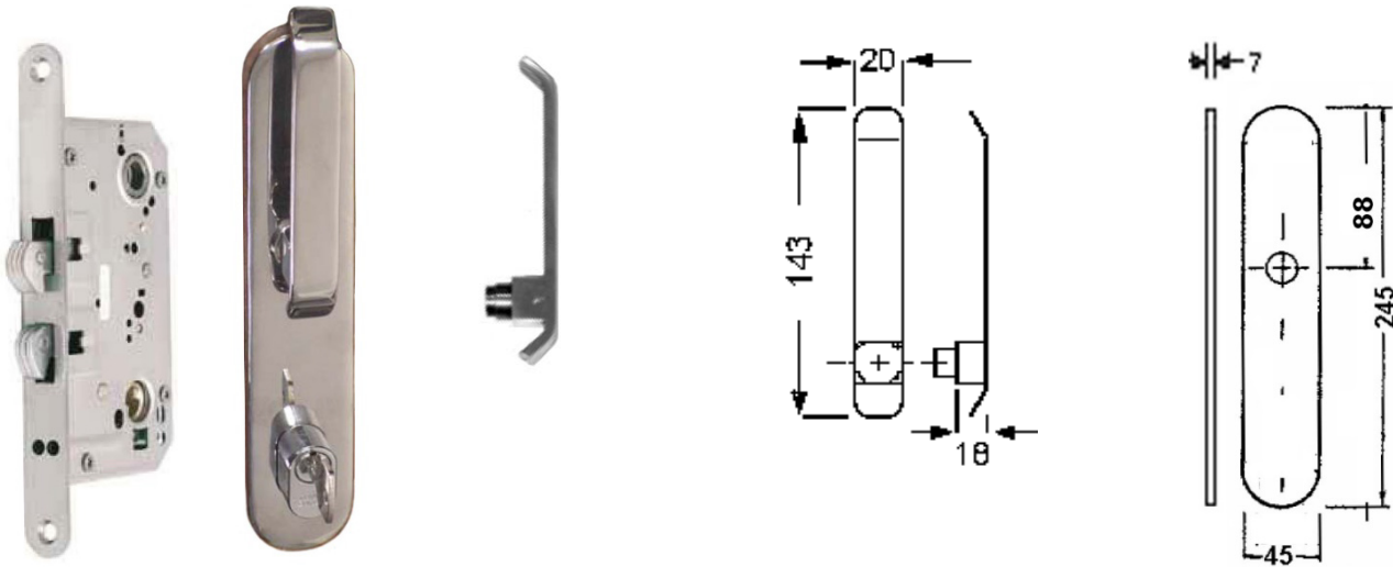
#11.SEFT.037 Complete sliding door lock, strike and key/thumb-turn
