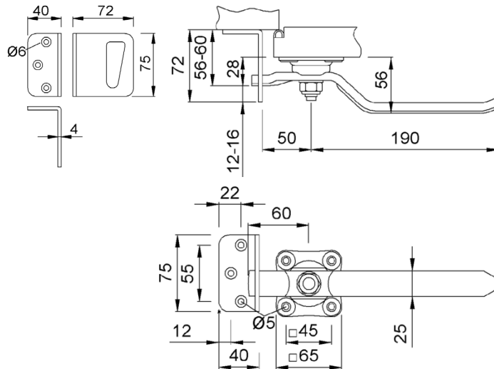
#44.130.508 Medium duty 304 stainless steel door dogging device 90 degree turn only
