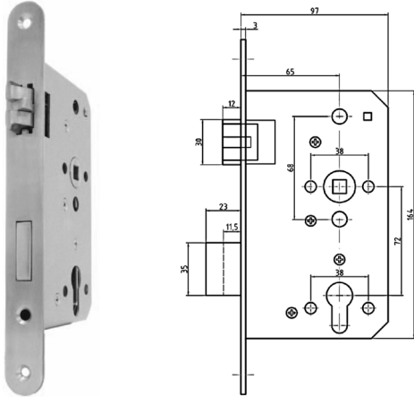
#14.3127.208 Entry Lock
