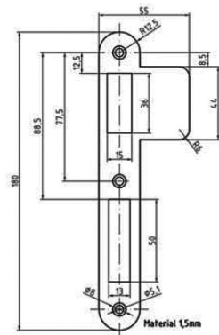
#14.0031.208 Strike Plate
