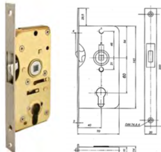
14.69Z entry sliding locks
