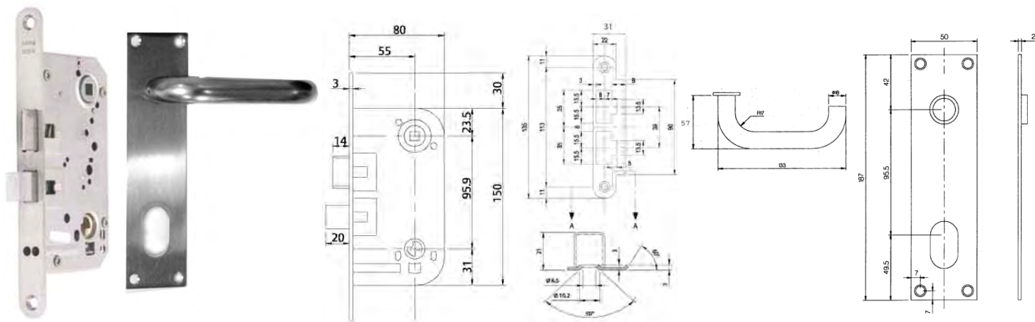
#11.SEET01. Complete Entry Lock Set Heavy Duty with stainless steel trim with escutcheon plates. Specify door thickness when ordering.
