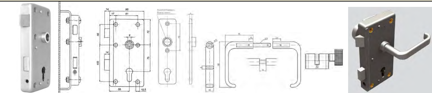
SET #13.27CZ Entry rim lock set complete; backset 55 mm Order Strike Box #13.225 SEPARATE
