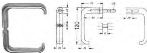
14.999 levers for rectangular escutcheon
