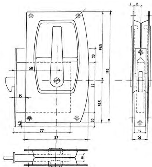
#18.3796 Passage sliding door lock 60 mm backset for minimum door thickness
