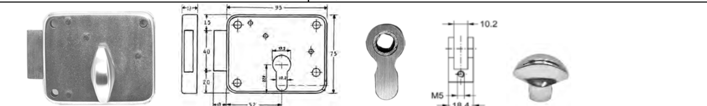
Rim lock #13.31SZ7; SET Deadbolt rim lock Privacy set with Thumb-turn. Backset 52 mm (2 inch). with thumb-turn #05.008
