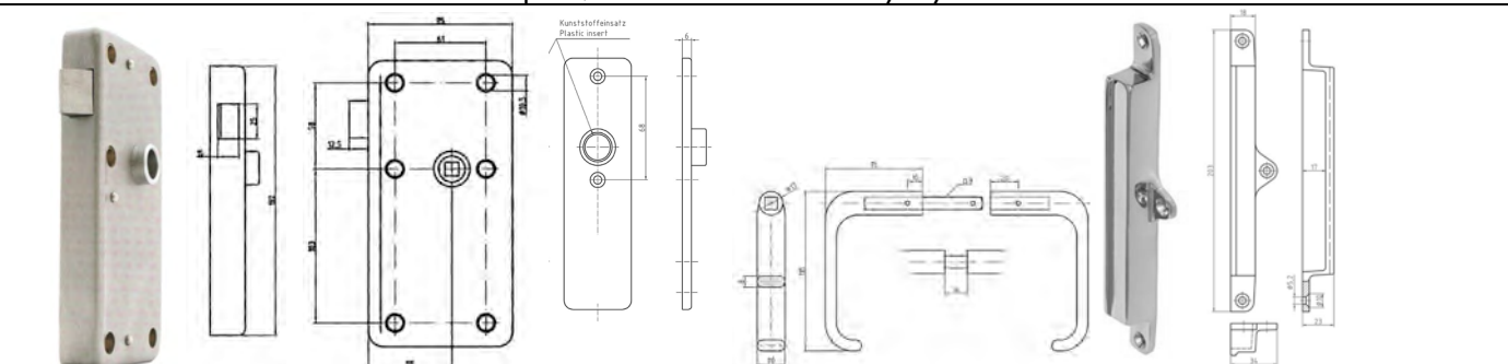
SET #13.27SF Passage rim latch set complete; backset 55 mm Order Strike Box #13.225 SEPARATE
