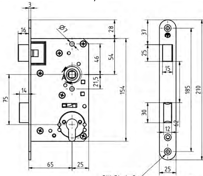
#14.4610.508 65 mm backset. Satin or Polished Stainless Steel
