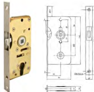
14.69W privacy sliding lock
