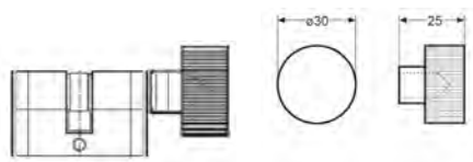
Profile Cylinder key/knob Series #05.405.566 for 1 1/2" thick doors
