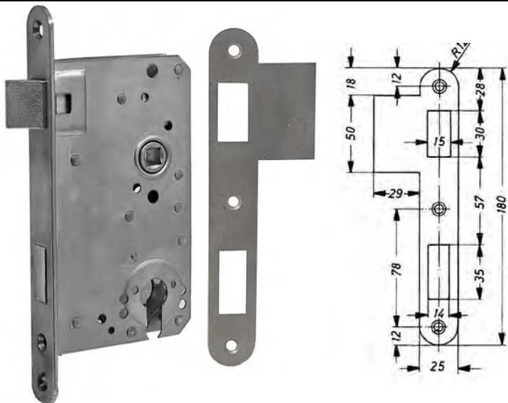
#14.4610.508 Heavy Duty Stainless Steel 65 mm backset Weather Door Entry Lock with solid latch bolt
