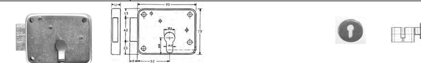
SET Rim lock #13.31Z.508 Deadbolt rim lock set complete; Backset 52 mm. Throw: 13 mm
