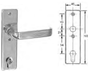
14.129 escutcheons for profile cylinder
