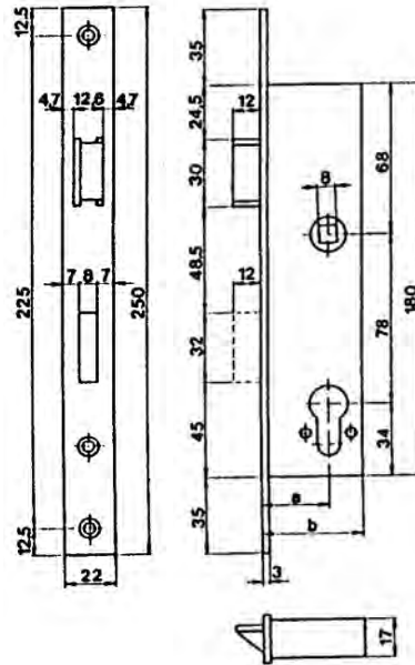
#19.82Z25.508 Narrow backset mortise entry lock lock case: 1 9/16 x 7 1/8" x 3/4" thick lock plate: 7/8" x 9 7/8" #12.021 Special cropped stainless steel lever handle with oval roses #12.507 Profile cylinder #05.400 with over roses #12.517
