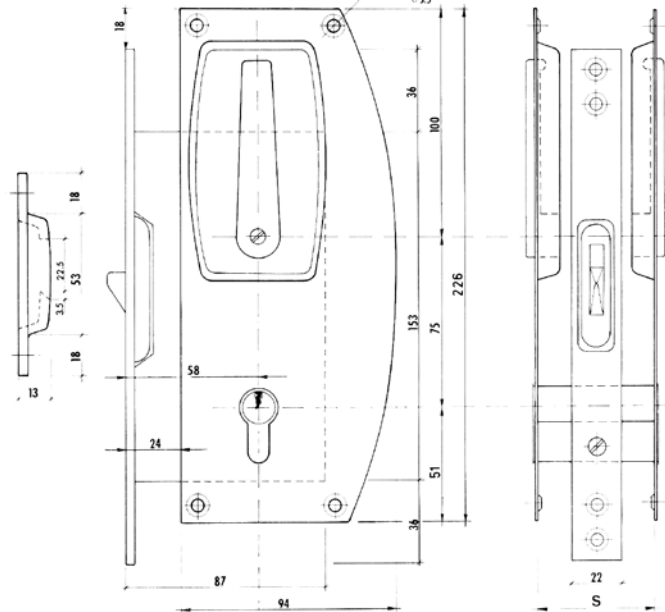
#18.3786 SET Entry Sliding door lock with Profile cylinder and strike box Min. door thickness: 38 mm or 1 1/2 inch
