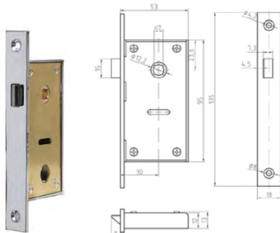
#18.68F Passage Latch
