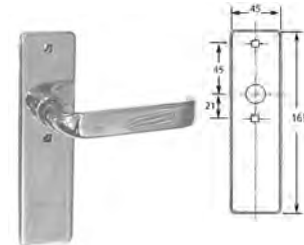
14.109 Escutcheons for passage lock
