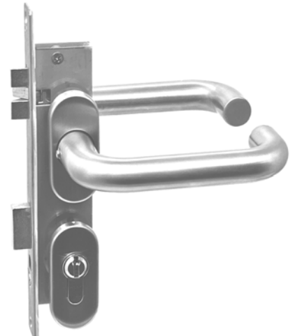
#19.82Z25.508 Narrow backset mortise entry lock lock case: 1 9/16 x 7 1/8" x 3/4" thick lock plate: 7/8" x 9 7/8" #12.021 Special cropped stainless steel lever handle with oval roses #12.507 Profile cylinder #05.400 with over roses #12.517
