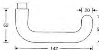
#11.SRFT.021 Complete privacy lock set with Lever #11.045 Lever with rose convex #12.110C
