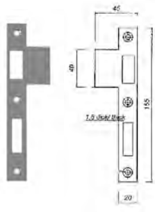
16.26Z Entry strike
