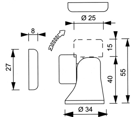
Magnetic doorholder #34.252.266 Polished Chrome Finish; Light duty for light weight doors Magnetic doorholder #34.252.566 Satin Chrome Finish; Light duty for light weight doors Magnetic doorholder #34.252.106 Polished Brass Finish; Light duty for light weight doors
