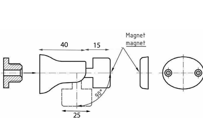
Magnetic doorholder #34.252.266 Polished Chrome Finish; Light duty for light weight doors Magnetic doorholder #34.252.566 Satin Chrome Finish; Light duty for light weight doors Magnetic doorholder #34.252.106 Polished Brass Finish; Light duty for light weight doors
