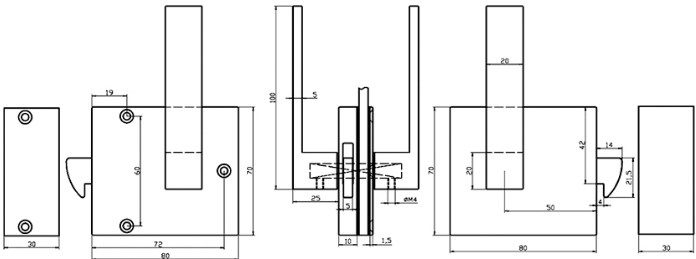
#81.8808 Glass or Wood Sliding Rim lock w. Strike Box. 1/4 to 1/2 inch thick glass and up to 3/4 inch wood. Chrome Plated Brass
